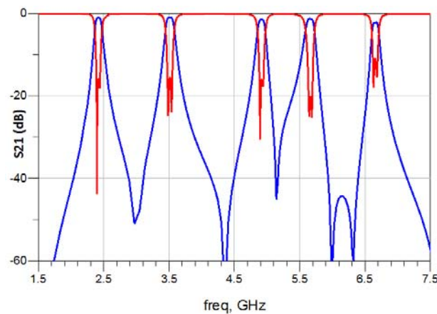
Fig. 10. Simulated insertion-loss and return-loss response of the proposed filter.
