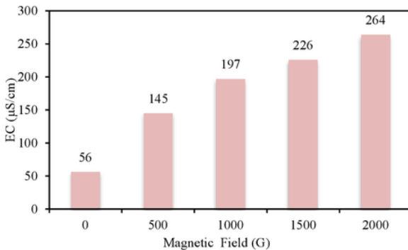
Fig. 7. Concentration of EC with magnetic filed.
