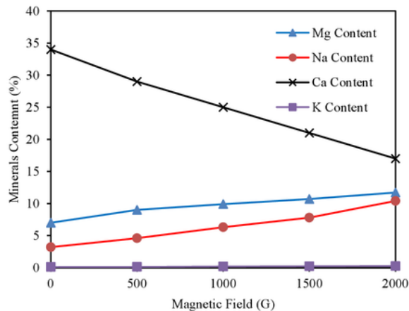
Fig. 4. Concentration of Mg with magnatic filed.
