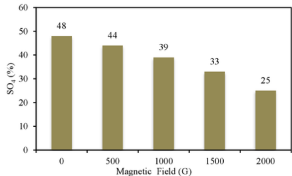
Fig. 9. Concentration of \text{SO}_4 with magnetic filed.
