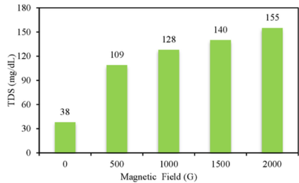
Fig. 8. Concentration of TDS with magnetic filed.
