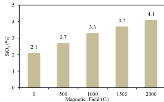
Fig. 6. Concentration of \text{SiO}_2 with magnatic filed.
